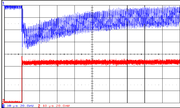
Figure 45. Typical Transient response: 5.0VIN,2.0VOUT.
