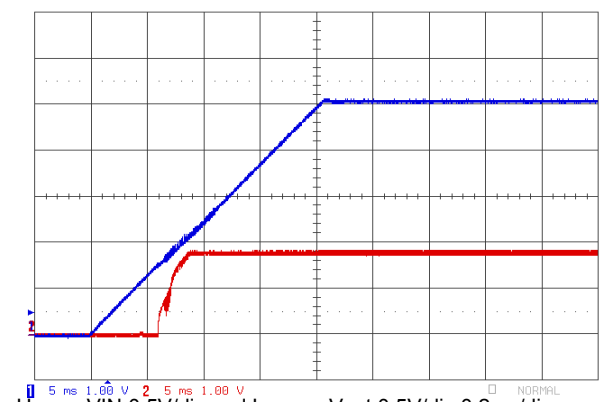
Upper=VIN 0.5V/div and Lower= Vout 0.5V/div 0.2ms/div Figure 32. Input/Output Start-Up Characteristics : 5.0VIN,1.8VOUT,20ms input ramp.
