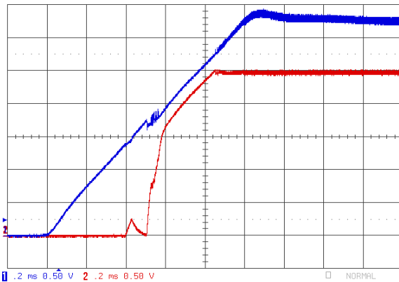
Upper=VIN 0.5V/div and Lower= Vout 0.5V/div 0.2ms/div Figure 27. Input/Output Start-Up Characteristics : 3.3VIN,2.5VOUT,1ms input ramp.
