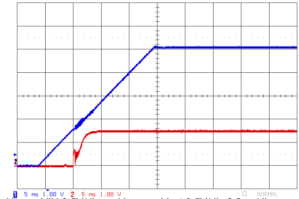
Upper=VIN 0.5V/div and Lower= Vout 0.5V/div 0.2ms/div Figure 30. Input/Output Start-Up Characteristics : 5.0VIN,1.5VOUT,20ms input ramp.
