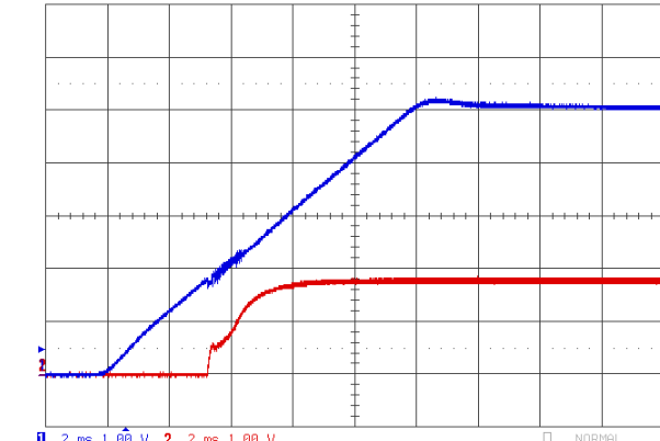
Upper=VIN 0.5V/div and Lower= Vout 0.5V/div 0.2ms/div Figure 31. Input/Output Start-Up Characteristics : 5.0VIN,1.8VOUT,1ms input ramp.
