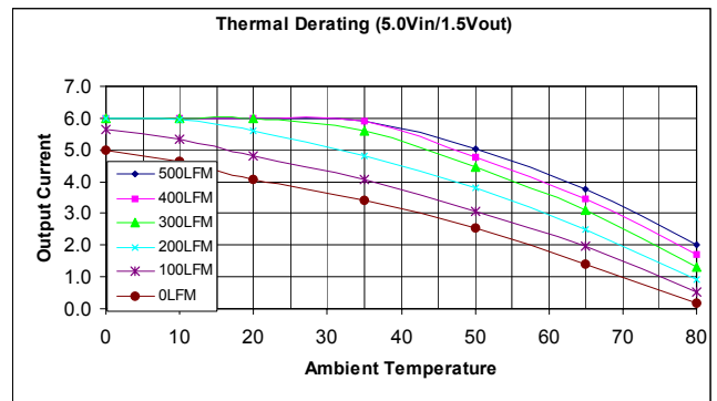
Figure 52. Thermal Derating for 5.0VIN ,1.5VOUT.
