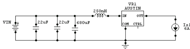
Figure 57. Input Reflected Ripple Current Test Setup.
