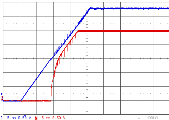
Upper=VIN 0.5V/div and Lower= Vout 0.5V/div 0.2ms/div Figure 28. Input/Output Start-Up Characteristics : 3.3VIN,2.5VOUT,20 ms input ramp.
