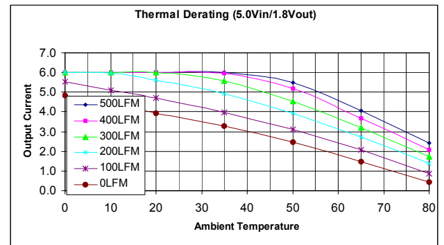
Figure 53. Thermal Derating for 5.0VIN ,1.8VOUT.
