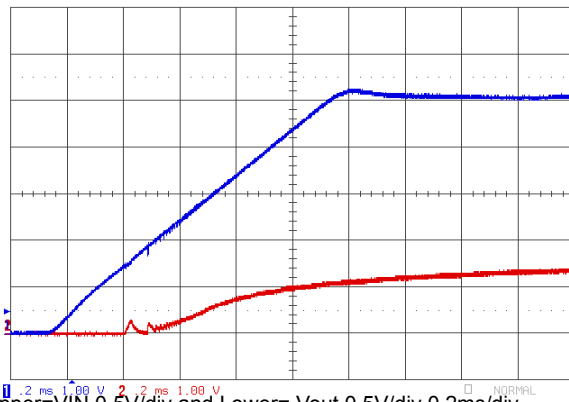
Upper=VIN 0.5V/div and Lower= Vout 0.5V/div 0.2ms/div Figure 29. Input/Output Start-Up Characteristics : 5.0VIN,1.5VOUT,1ms input ramp.
