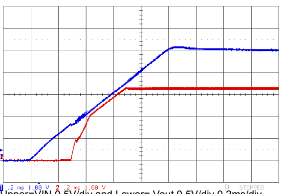
Upper=VIN 0.5V/div and Lower= Vout 0.5V/div 0.2ms/div
