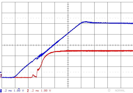
Upper=VIN 0.5V/div and Lower= Vout 0.5V/div 0.2ms/div
