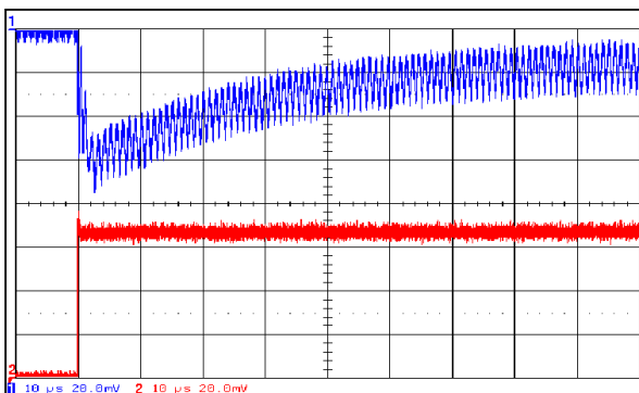
Blue(upper)=Vout 20mV/div Red(lower)=1A/div 10µs/div
