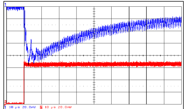
Blue(upper)=Vout 20mV/div Red(lower)=1A/div 10µs/div
