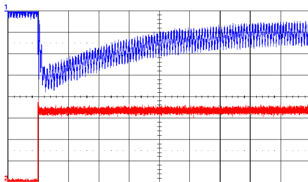
Blue(upper)=Vout 20mV/div Red(lower)=Vin1A/div 10µs/div
