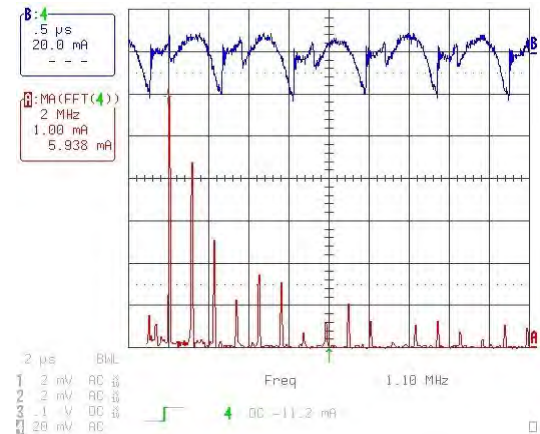
Figure 11. Typical Input Reflected Ripple current 5.0VIN, 3.3VOUT.
