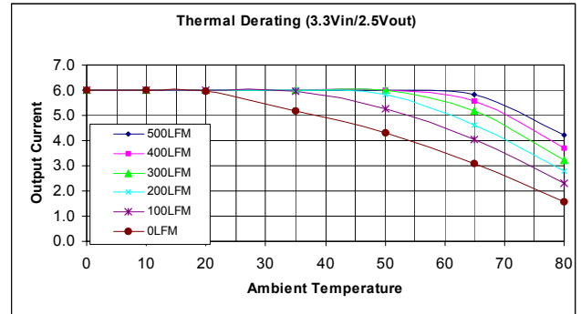
Figure 51. Thermal Derating for 3.3VIN ,2.5VOUT.
