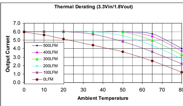
Figure 49. Thermal Derating for 3.3VIN ,1.8VOUT.
