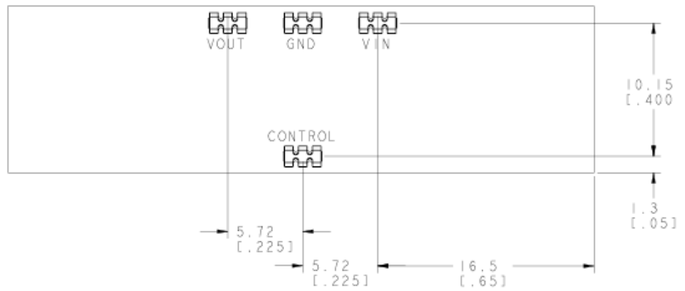
Bottom View
